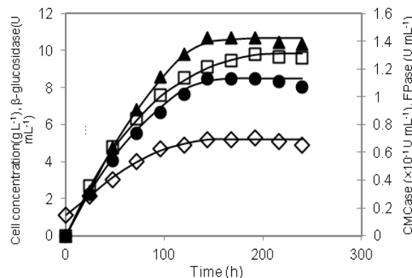
Fig. 1 Comparison between the calculated and experimental data for shake-flask fermentation of cellulase by A. terreus . \diamond , Cell concentration; \bullet , FPase activity; \blacktriangle , CMCase
