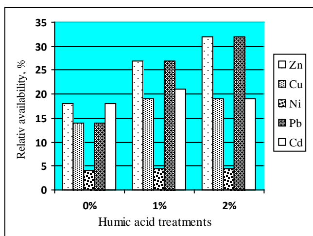
Fig. 1. Effect of the application of humic acid to soil relative availability of heavy metals
