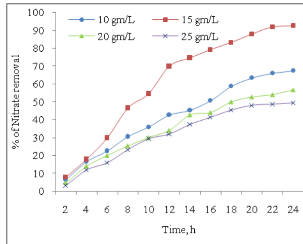
Fig.2 Percentage of nitrate removal at 150 mg/L using Poly propylene biofilm carriers
